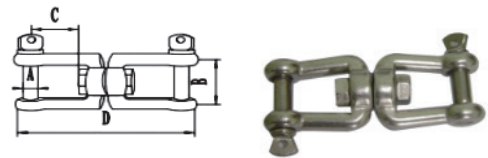
SWIEL JAW JAW 叉叉式链接转环
