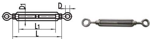
TURNBUCKLE TYPE EYE-EYE 开体花篮
