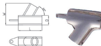
Tees with cable eyelet 60° 60度带缆孔三通
