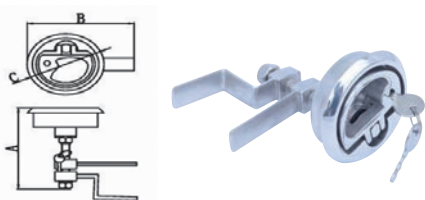
Turning Lock Lift Handle 地板锁
