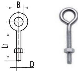
EYE BOLT WITH RING AND NUT 吊环螺丝
