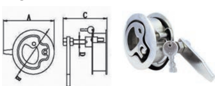
Turning Lock Lift Handle 地板锁
