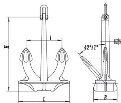
A type 矩形杆
