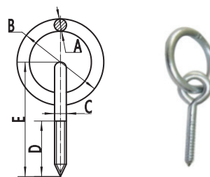
DOCK RING(CARBON STEEL) 码头环
