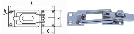
Eccentric Latch 搭扣
