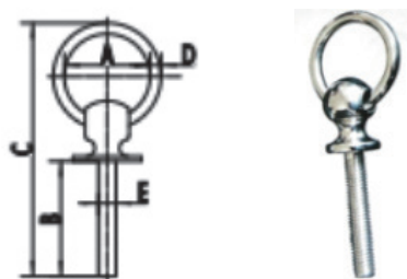
LIFE SAVING RING 救生环
