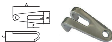
Pothook 挂钩
