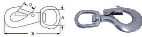
SWIVEL SNAP HOOK 万向钩
