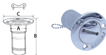
Deck filler in steel 加油口
