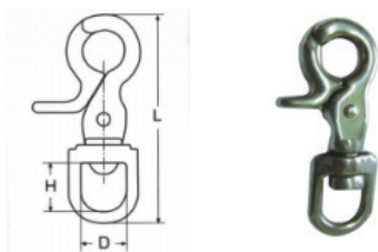
TRIGGER SNAP HOOK WITH SWIVEL EYE 挂钩
