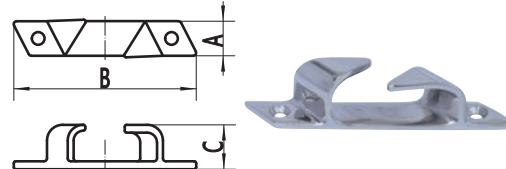
Skene Bow Chock 斜尖导缆器
