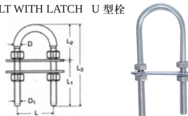
U BOLT WITH LATCH U 型栓
