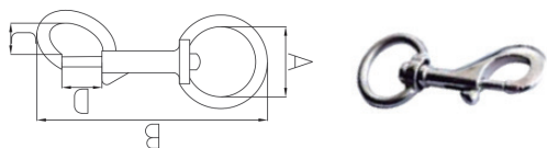
SWIVEL EYE SNAP 挂钩
