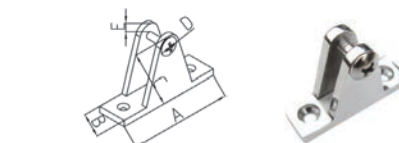
Deck hinge 90° concave base 栓式正山型座
