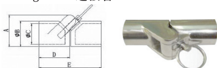
Swivelling Joints 连接管
