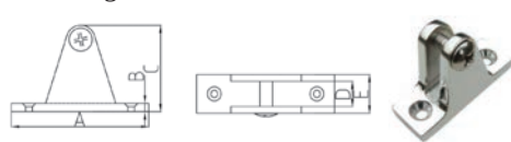
Deck Hinge Base-60° 60 度栓式山型座
