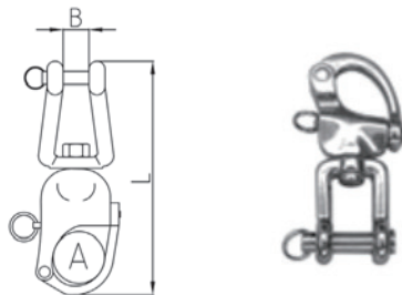
SWIVEL SNAP SHACLE WITH JAW 卸扣
