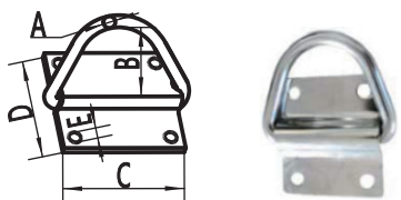
Dee Ring D 型环
