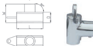
Tees with cable eyelet 90° 90度带缆孔三通
