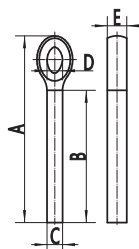
SHOULDER EYE BOLT 吊环螺母
