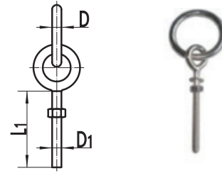
WELD EYE BOLT WITH RING AND NUT 吊环螺丝
