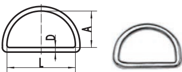
WELD D RING 焊接 D 型环
