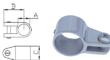
Tope Slide 滑套
