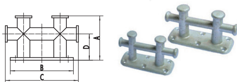
Hot Dipped Galvanized Double-Cross Bollard 碳钢双十字
