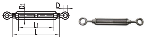
TURNBUCKLE TYPE EYE-EYE 开体花篮
