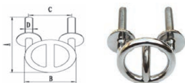
Water ski tow 滑水圈
