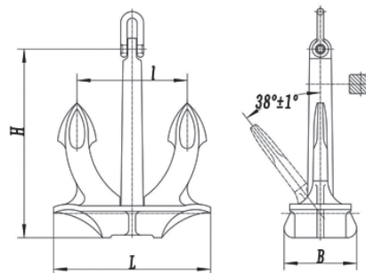
C type 矩形短杆
