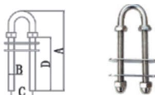
U-BOLT U 型栓
