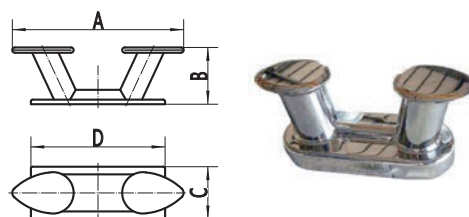
Horn Bollard 板凳
